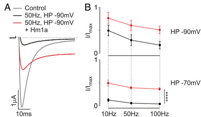
Fig. 3. Hm1a prevents frequency-dependent current reduction in available channels. (A) Representative current traces from oocytes expressing Na_v1.1 before stimulation (control, gray trace), and after 50-Hz simulated action potentials for 1 s at a holding potential (HP) of -90 mV in the absence (black trace) or presence (red trace) of 100 nM Hm1a. (B) Group data showing the availability of Na_v1.1 following the simulated action potentials at the rate and holding potential indicated. Hm1a significantly increases Na_v1.1 availability over a range of conditions. Values are shown as mean \pm SEM with n = 5 . P < 0.001 , two-way ANOVA.
