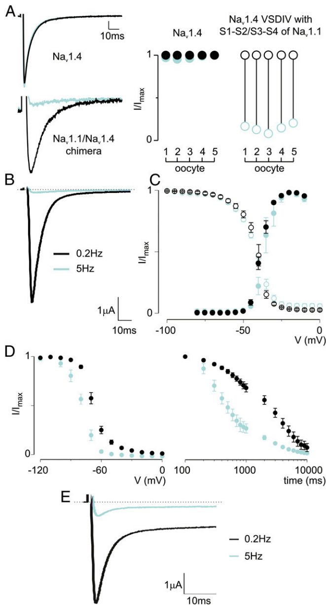
Fig. 4. ICA accelerates entry into slow inactivation without affecting fast inactivation. (A, Left) Representative current traces from oocytes expressing \text{Na}_v1.4 or \text{Na}_v1.4 containing the S1-S2/S3-S4 VSDIV loop of \text{Na}_v1.1 (black, control) in the presence (cyan) of 500 nM ICA-121431 during repeated stimulations from -90 mV to -10 mV at 5 Hz. (A, Right) Summary of current inhibition at -10 mV (holding -90 mV) as a result of applying 500 nM ICA-121431 on five oocytes expressing \text{Na}_v1.4 or \text{Na}_v1.4 containing the S1-S2/S3-S4 VSDIV loop of \text{Na}_v1.1 . (B) Representative current traces from oocytes expressing \text{Na}_v1.1 in the presence of 500 nM ICA-121431 during repeated stimulation from a -90 mV holding potential to -30 mV at the indicated rate. (C, Left) Voltage-activation relationship for \text{Na}_v1.1 in the absence (black) or presence (blue) of ICA (500 nM). The protocol was as shown in Fig. 3, except cells were held for 10 s at -90 mV between sweeps. The V_{1/2} of activation was -37 \pm 1 mV in the presence of ICA vs -38 \pm 1 mV in the absence of ICA. This shift did not reach statistical significance ( P > 0.05 , Student's t test). (C, Right) SSI curve for which cells were held for 10 s at -90 mV between sweeps. Values are shown as mean \pm SEM with n = 6 . (D, Left) Voltage dependence of slow inactivation in the absence and presence of ICA (500 nM) using a protocol similar to that shown in Fig. 2. (D, Right) Time-dependence of entry into slow inactivation according to the protocol in Fig. 2. Values are shown as mean \pm SEM with n = 6 . (E) Currents elicited during stimulation as indicated in the presence of both ICA (500 nM) and Hm1a (500 nM).
