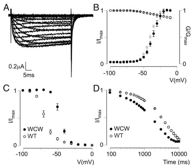
Fig. 5. \text{Na}_v1.1 WCW affects fast and slow inactivation. (A) Representative family of current traces from oocytes expressing the \text{Na}_v1.1 WCW mutant exposed to various activating voltages from -100 to 0 mV. As illustrated, fast inactivation is removed. (B) Activation-voltage (solid symbols, calculated G/G_{\text{max}} ) and SSI (open symbols, I/I_{\text{max}} ) relationships of \text{Na}_v1.1 WCW. Also shown in gray is the activation-voltage relationship obtained from measuring tail currents ( I/I_{\text{max}} ). The V_{1/2} for this curve ( -39 \pm 1 mV) is similar to that obtained from the calculated activation-voltage relationship. Values are shown as mean \pm SEM with n = 4 . (C) Voltage dependence of slow inactivation for \text{Na}_v1.1 WCW (filled circles) compared with WT \text{Na}_v1.1 (open circles). Values are shown as mean \pm SEM with n = 4 . (D) Entry into slow inactivation for \text{Na}_v1.1 WCW (filled circles) compared with WT \text{Na}_v1.1 (open circles). Values are shown as mean \pm SEM with n = 4 .
