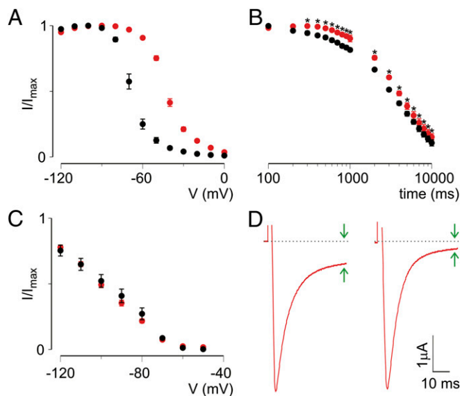
Fig. 2. Hm1a inhibits entry into the slow inactivated state. (A) Voltage dependence of slow inactivation in the absence (black) or presence (red) of 1 \mu M Hm1a (filled circles). Oocytes were held at -90 mV and exposed to the different conditioning voltages for 10 s, followed by a -100 -mV pulse for 50 ms to remove fast inactivation and then a test pulse to -20 mV. V_{1/2, control} = -68 \pm 2 mV; V_{1/2, Hm1a} = -42 \pm 1 mV for Hm1a. Hm1a significantly shifts the V_{1/2} of slow inactivation. Values are shown as mean \pm SEM with n = 5 . P < 0.001 , Student's paired two-tailed t test. (B) Kinetics of entry into the slow inactivated state in the absence (black) or presence (red) of Hm1a (1 \mu M). Oocytes were held at -90 mV and pulsed to -20 mV for various durations, followed by a 50-ms pulse to -100 mV to recover channels from fast inactivation and a test pulse at -20 mV for 50 ms. Entry into slow inactivation is significantly slower in the presence of Hm1a across a range of durations (300 ms–10 s; indicated with an asterisk). Values are shown as mean \pm SEM with n = 5 . P < 0.01 , two-way ANOVA with Tukey's post hoc test. (C) Recovery from slow inactivation in the absence (black) or presence (red) of Hm1a (100 nM). Oocytes were held at -90 mV and exposed to -20 mV for 10 s, pulsed to -100 mV for 200 ms, then held at various recovery voltages for 10 s before a test pulse at -30 mV. Data are normalized to the peak current at -30 mV assayed before recovery from the slow inactivation protocol. Values are shown as mean \pm SEM with n = 5 . (D) Representative current traces before (Left) and after (Right) recovery from the slow inactivation protocol as in C.
